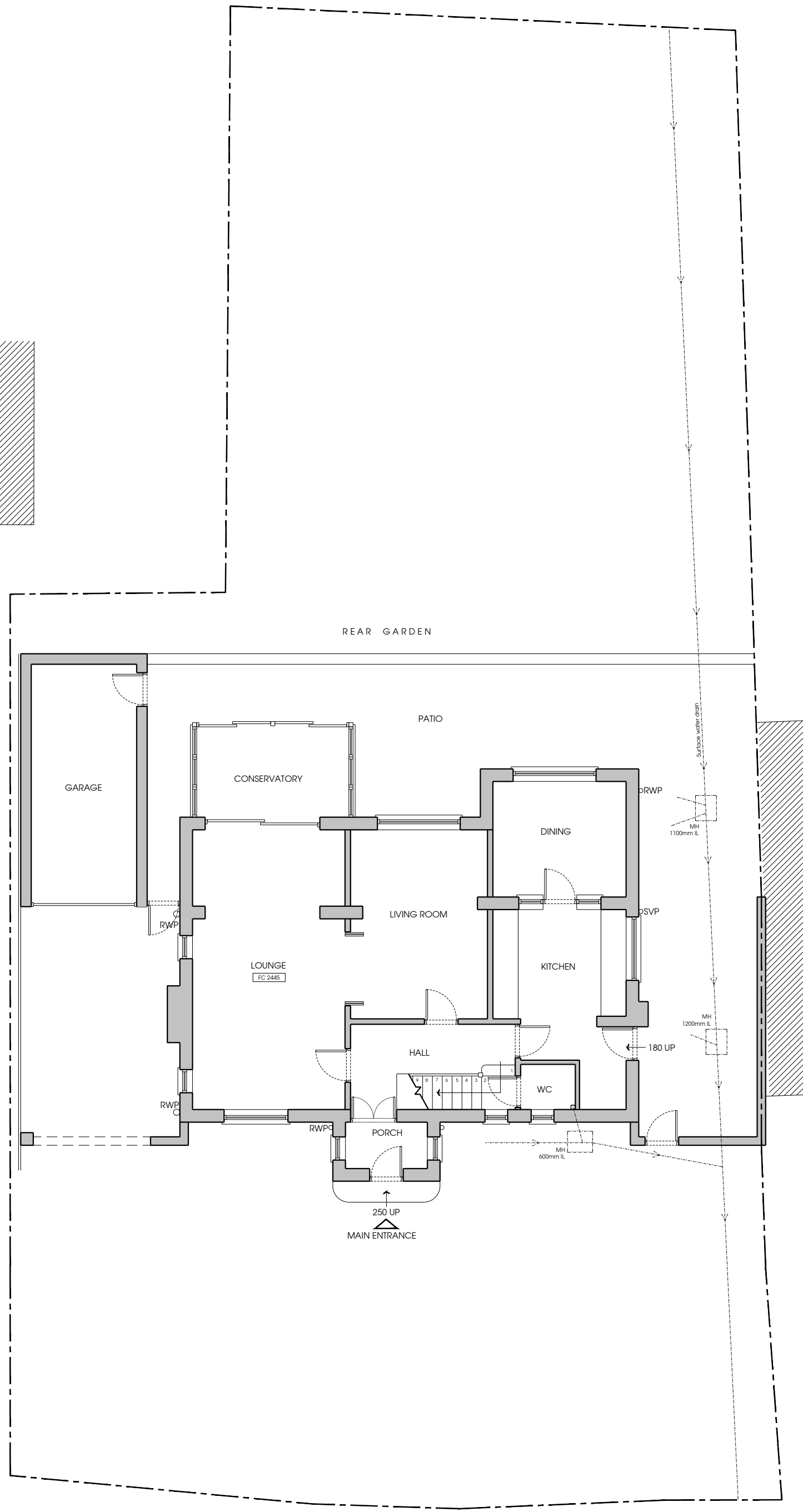
03 EXISTING GROUND FLOOR PLAN 1 : 100
